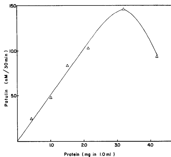
FIG. 4. Protein Dependence of Patulin Synthesis. Assays were performed as described in the text varying the protein concentration over the range shown. ATP was not added to the incubations.
