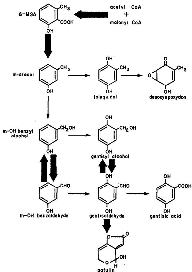
SCHEME I. The Pathway of Patulin Biosynthesis. (Darker arrows represent biosynthetic conversions which have been demonstrated enzymatically by this study or previous studies.)
