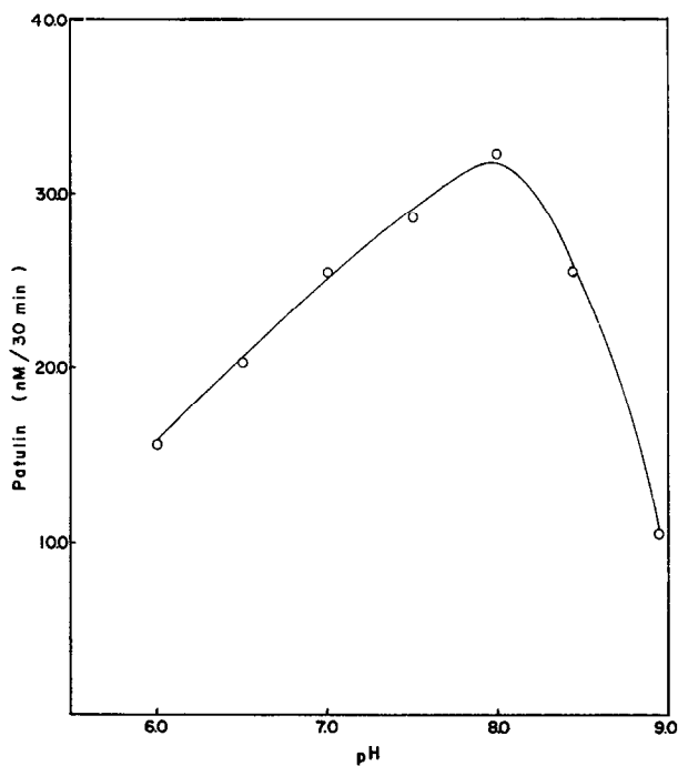
FIG. 5. pH Dependence of Patulin Synthesis. The pH of the incubation mixture was adjusted with 0.1M HCl or 0.1M NaOH. The reaction was started by the addition of substrates (0.2 \mu M ^{14} C gentis-aldehyde, 1.0 \mu M NADPH, 1.0 \mu M ATP) and assayed as described in the experimental methods.
