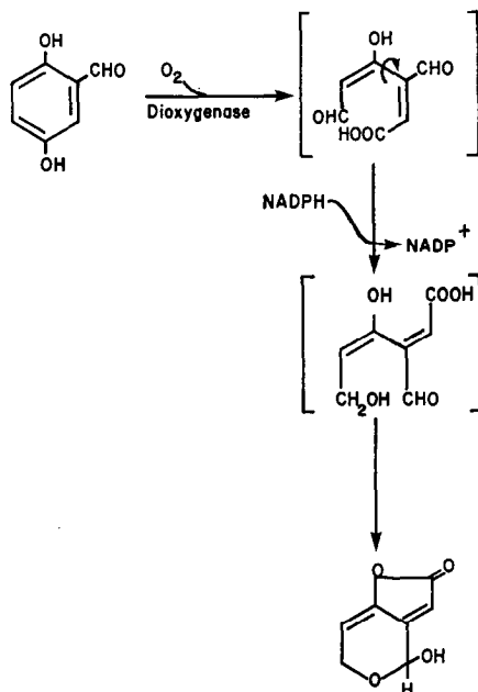
SCHEME II. The Proposed Mechanism of Patulin Biosynthesis from Gentisaldehyde. [Brackets indicate proposed intermediates.]
