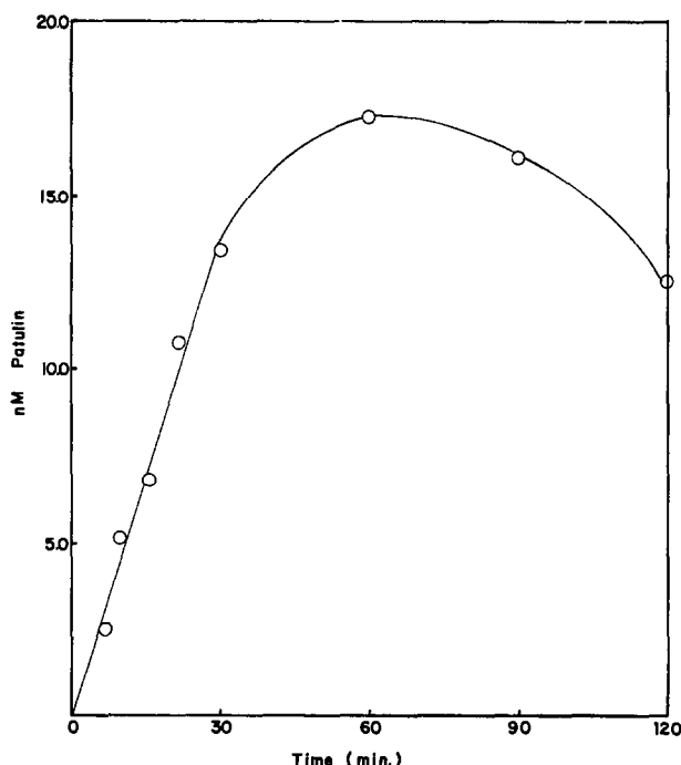
FIG. 3. Time Dependence of Patulin Synthesis. The enzyme assays were performed as described in the experimental procedure using 2.5 mg of protein (100,000g supernatant) except the time was varied and ATP was not added.
