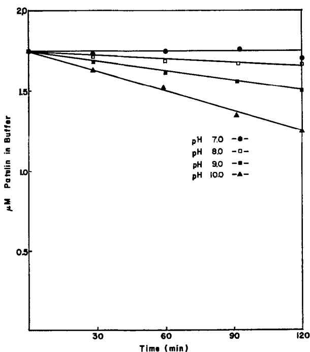
FIG. 6. Stability of Patulin at Various pH's. 0.025 ml of a 10 mg/ml solution of patulin was added to 1.0 ml of 0.1N tris-HCl buffer of different pH's and incubated at 28°C. 0.10 ml of the buffer-patulin solution was assayed at various times by placing it in 2.9 ml of 0.1N HCl in a uv cell. The O.D. at 276 nm was measured and the amount of patulin remaining in the buffer was calculated using 13,350 as the molar extinction coefficient of patulin at 276 nm.
