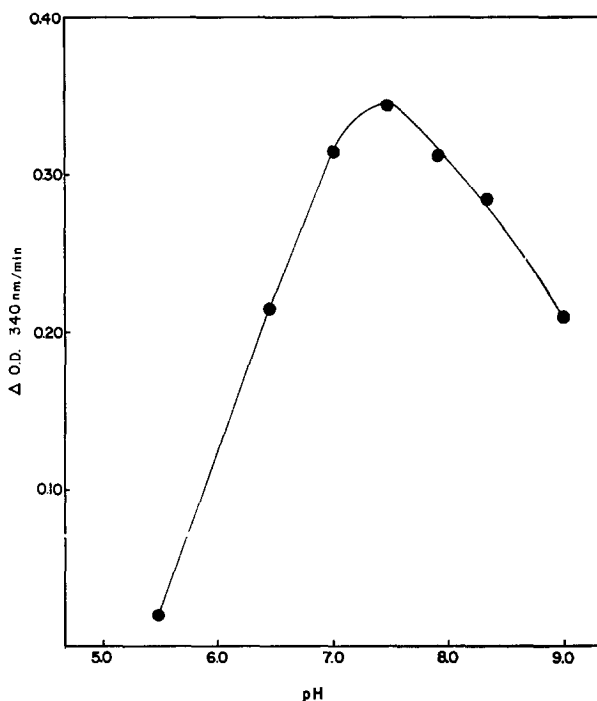
FIG. 2. pH Dependence of Dehydrogenase activity. The pH of the incubation mixture was adjusted with 0.1M HCl or 0.1M NaOH. The assays were performed by the optical method.
