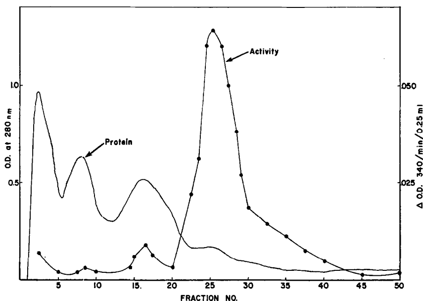
FIG. 1. DEAE Cellulose Chromatography of Dehydrogenases. The procedure is described in the text.
